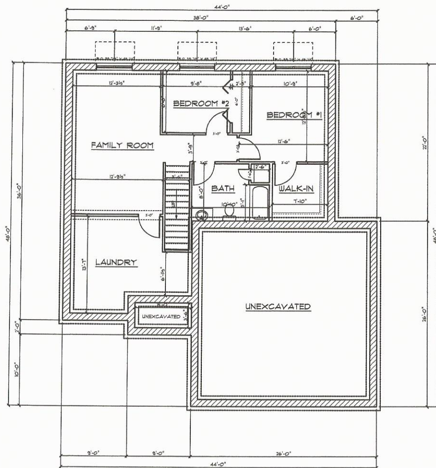
BASEMENT PLAN
